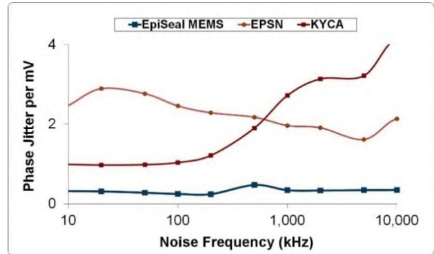
Figure 6. Shock Robustness [6]
